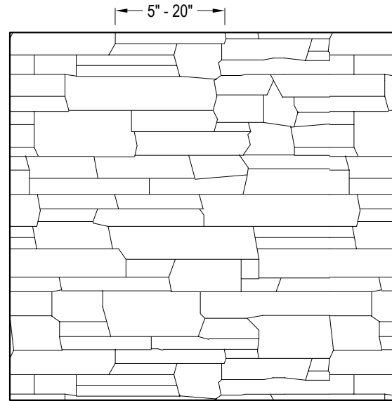
FRONT ELEVATION - DESIGNER CUT
