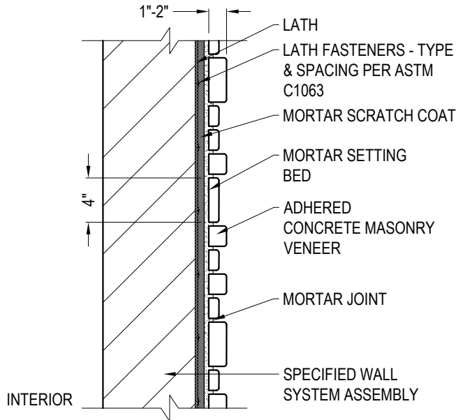
TYPICAL SECTION
