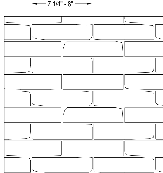
FRONT ELEVATION - PLYM BRICK
