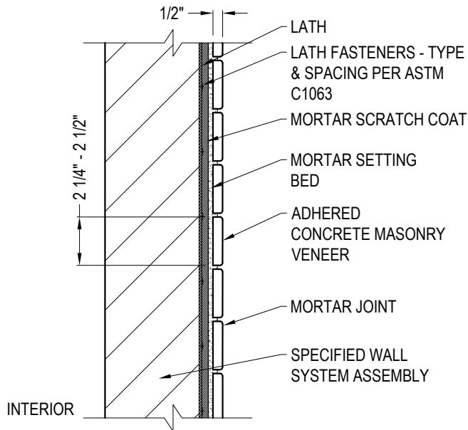
TYPICAL SECTION
