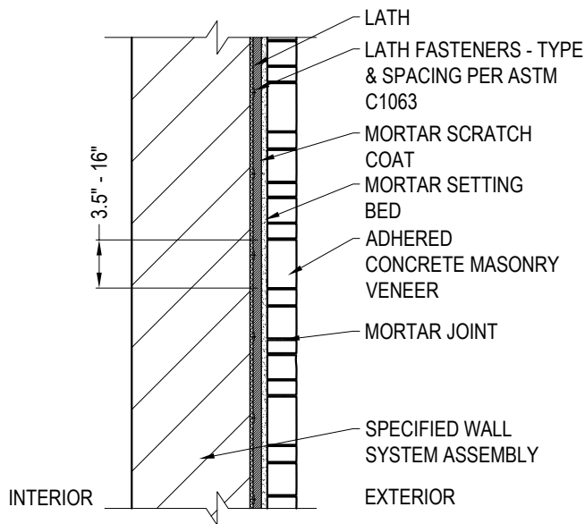
TYPICAL SECTION
