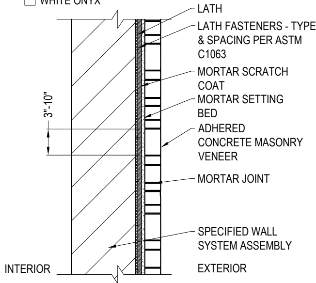
TYPICAL SECTION
