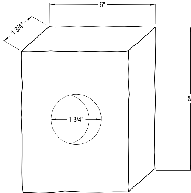
PERSPECTIVE WATER HYDRANT BLOCK
