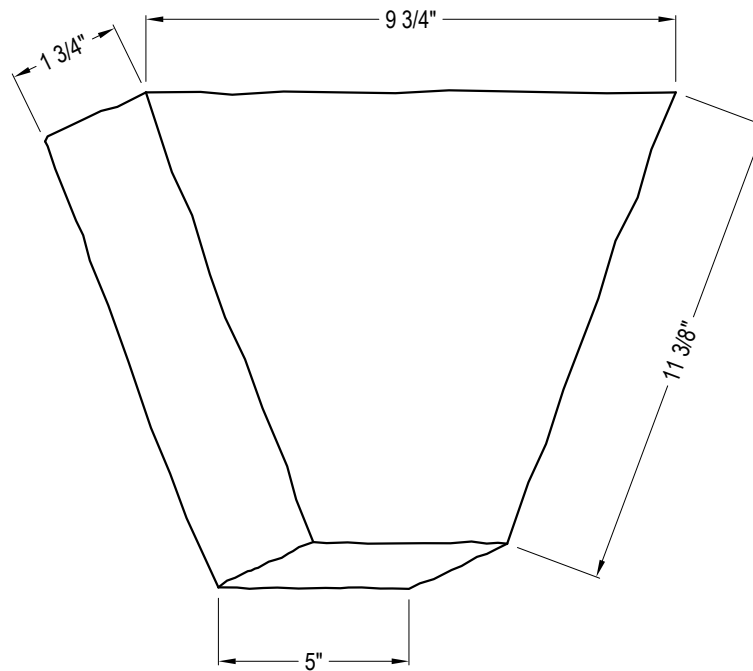
PERSPECTIVE ROCKFACE KEYSTONE
