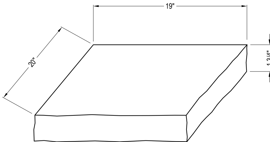
PERSPECTIVE HEARTHSTONE
